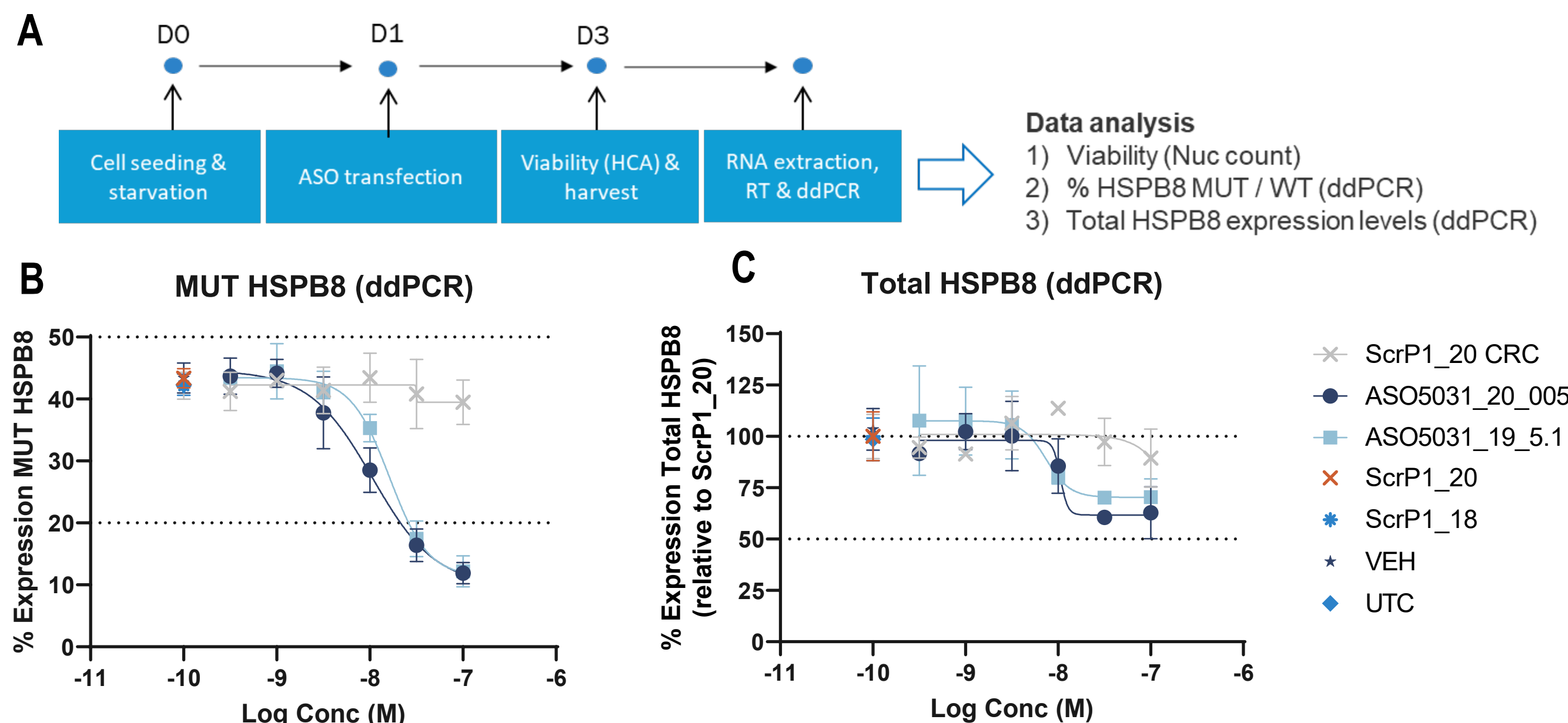
FIGURE 1: Experimental workflow for ASO screening in patient fibroblasts using transfection (Fig. 1A). Results from the potency determination of 2 top ASO hits in 6-point concentration-response curves (100 nM top concentration, half-log dilution steps) showed a 72% reduction in MUT HSPB8 at the top concentration (Fig. 1B). A comparable reduction in the total HSPB8 RNA levels indicate good selectivity (Fig. 1C)
