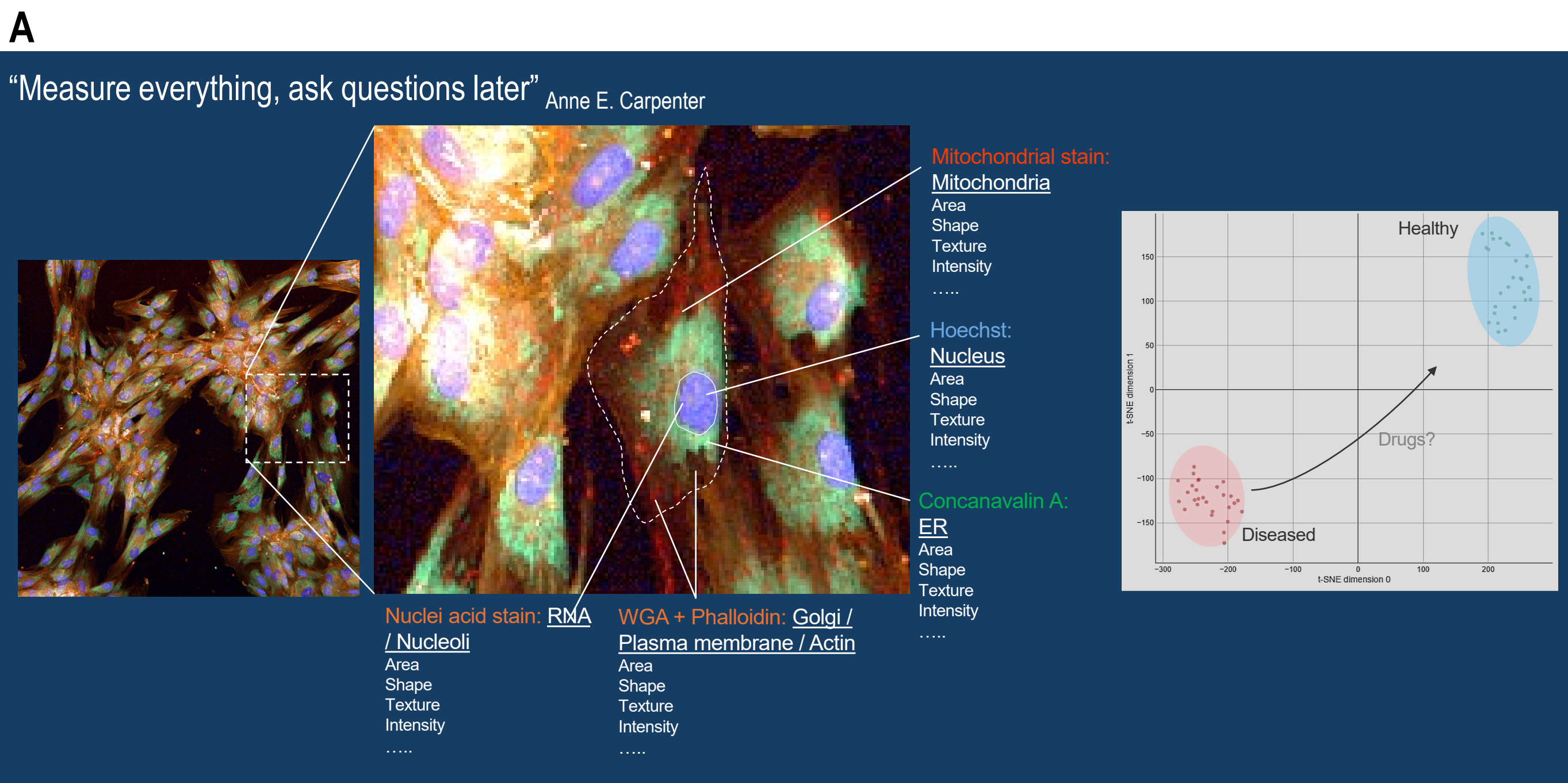
FIGURE 2: Cell Painting assay for phenotypic high-content screening (Fig. 2A). Experimental workflow for compound screening in patient fibroblasts (Fig. 2B). Quality control of the Machine Learning (ML) model performance showing the % cells classified as healthy from patient and healthy DMSO-treated control wells (Fig. 2C). Results from the drug repurposing screen at 10 µM are shown in a correlation plot where each point represents the % healthy cells per well, with replicate 1 on the X-axis and replicate 2 on the Y-axis. The 120 hit compounds selected for validation and potency determination included several different drug classes and >70 targets (Fig. 2E). The two best ASOs were also tested in the CP assay at 100 nM and 31.6 nM for 72h to assess phenotypic changes, but there were no effects in the ML results. However, Principal Component Analysis (PCA) showed morphological differences at 100 nM in dimension 1, mostly related to Mitochondrial features (Fig. 2F).
